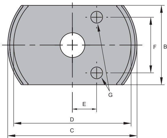
Magnet Shim
