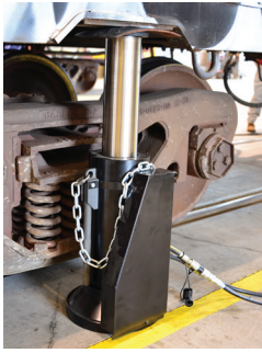
◀ Rail Car Jack, JDR80, lifting the back of a rail car for the operator to start maintenance on the car's wheels.
